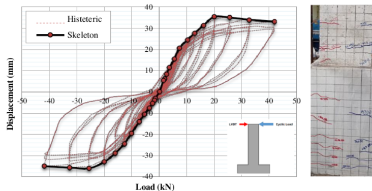
Figure 7. Hysteresis curve specimen KR02
