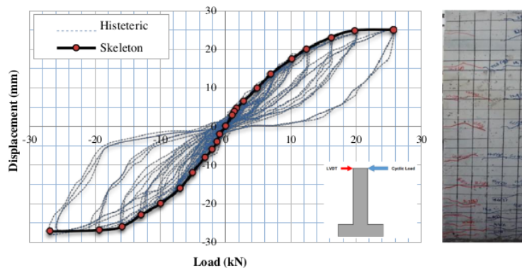
Figure 5. Hysteresis curve specimen KK
