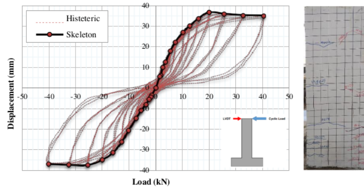
Figure 6. Hysteresis curve specimen KR01
